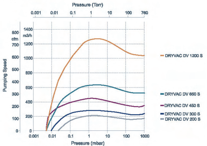
Pumping speed curves
